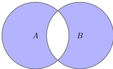
A \Delta B = (A \cap \bar{B}) \cup (B \cap \bar{A}) Symmetrische Differenz
