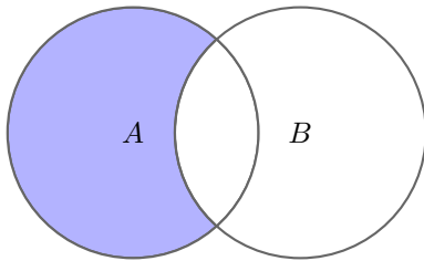
A \setminus B = A \cap \bar{B} Differenz
